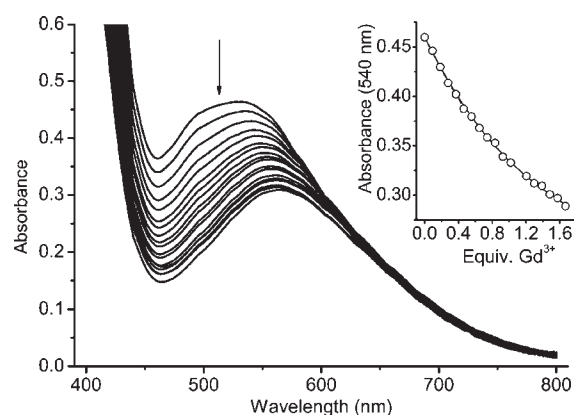
Figure 3. Experimental spectra for the titration of 4 ( \{\text{Ca}^{\text{II}}[15\text{-MC}_{\text{Cu}^{\text{II}}(\text{N})(\text{S})\text{-trpha-5}\}^{2+} ) with Gd 3+ in methanol/water 99:1 v/v solution ( C_{15\text{-MC-5}} = 1.01 \times 10^{-3} \text{ M} , Gd/Ca = 0–1.74, buffer MES 50 mM, pH 6.5). Inset: experimental (o) and calculated (line) values of the absorbance values at 540 nm.
